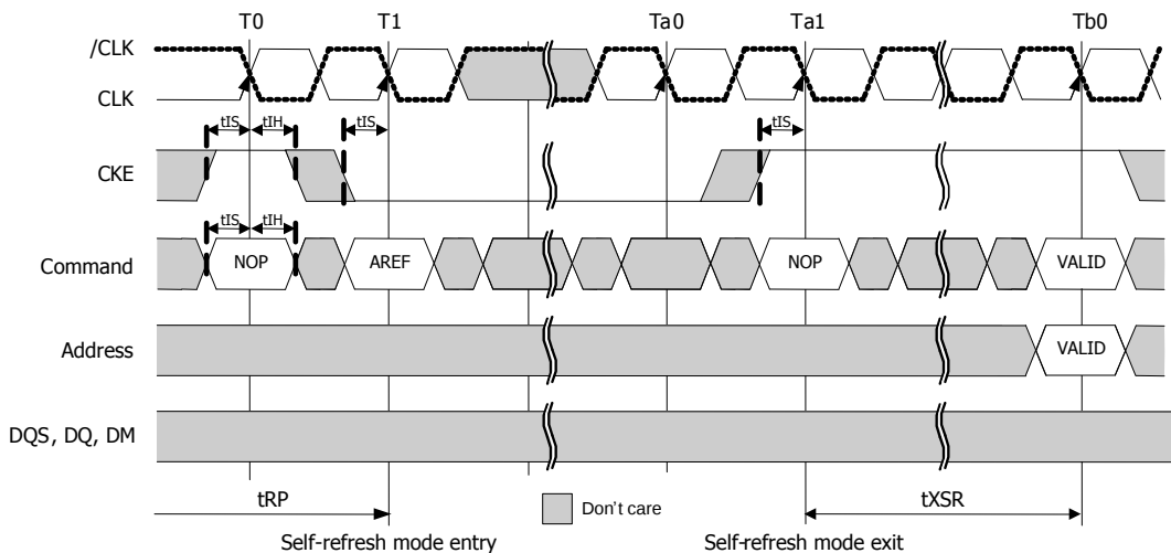
Figure35 : Self refresh
